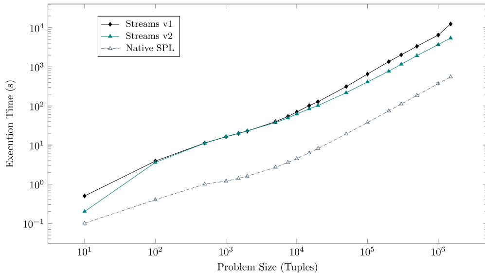
Fig. 10. Scalability Comparison of CRUCIBLE Online Runtimes and Native Implementations.
