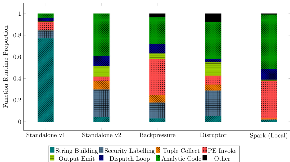
Fig. 4. Function runtime breakdown across Standalone Dispatchers.
